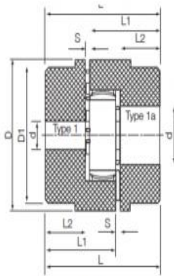
Curve Jaw Couplings (Pilot Bore)
