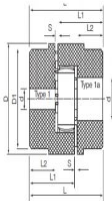
Curve Jaw Couplings (Pilot Bore)
