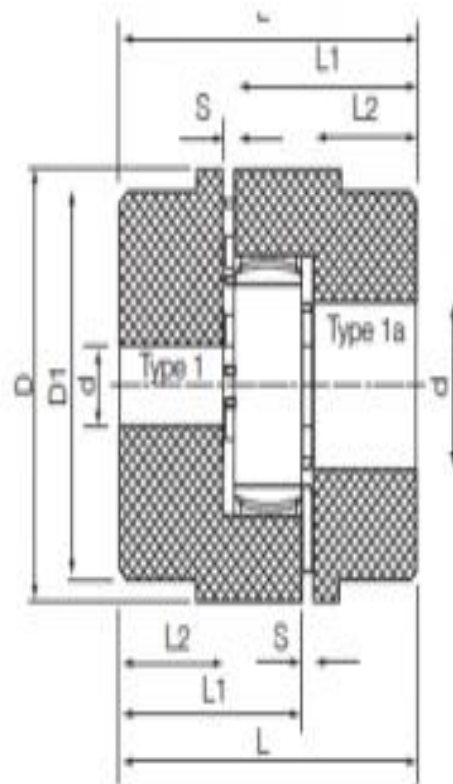
Curve Jaw Couplings (Pilot Bore)
