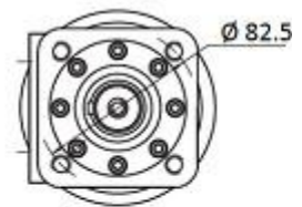
Q - Mount, 3/8 UNC 4 B
