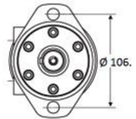
Standard Mount, SAE A
