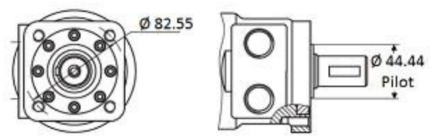
Q - Mount, 3/8 UNC 4 Bolt
