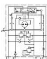
Closed Centre Load Sense using PRD/80 Valve
