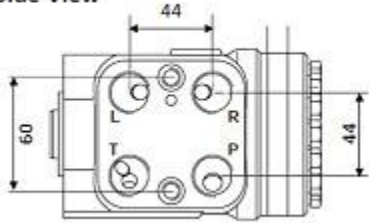
Standard Side View
