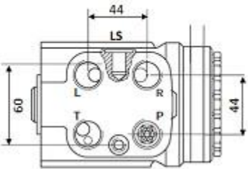
Load Sense Side View
