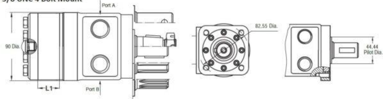
3/8 UNC 4 Bolt Mount
