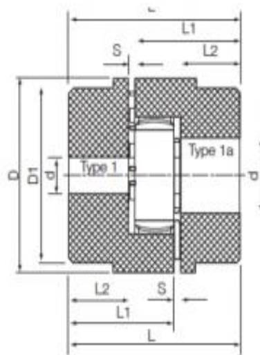
Curve Jaw Couplings (Pilot Bore)
