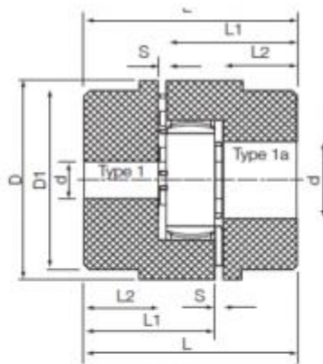
Curve Jaw Couplings (Pilot Bore)
