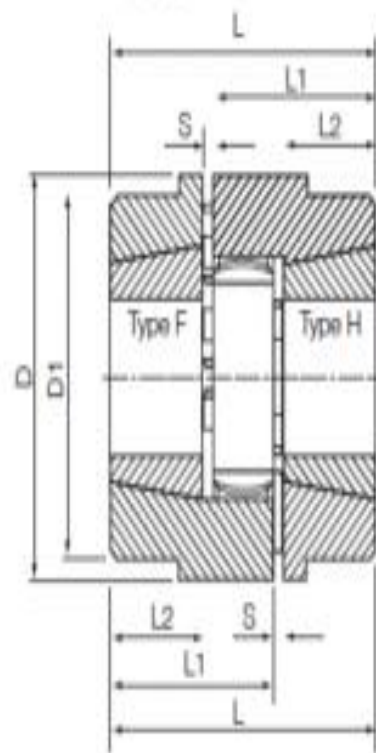
Curve Jaw Couplings (Taperlock)
