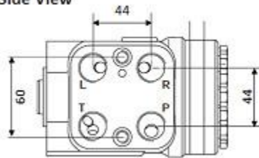
Standard Side View
