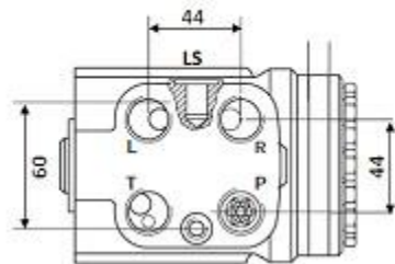
Load Sense Side View
