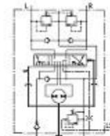
Closed Centre Load Sense Relief/Shock Valves
