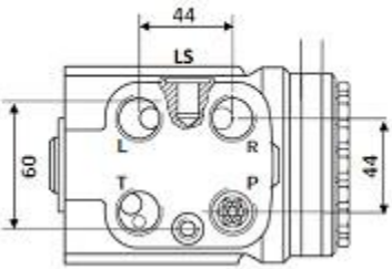
Load Sense Side View
