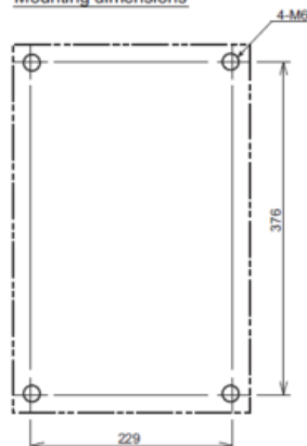
Mounting dimensions
